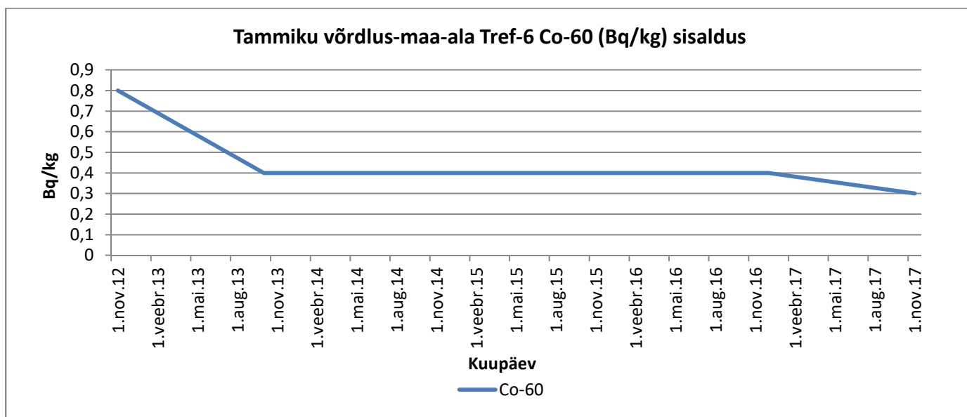
Graafik 102. Co-60
