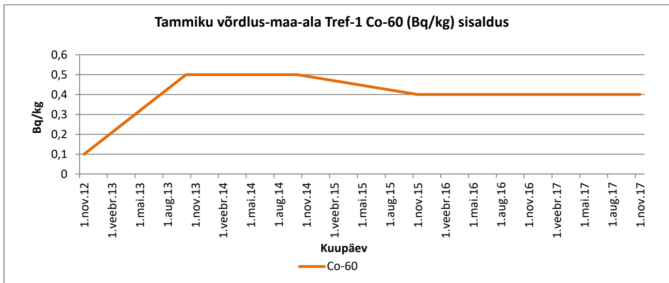
Graafik 72. Co-60
